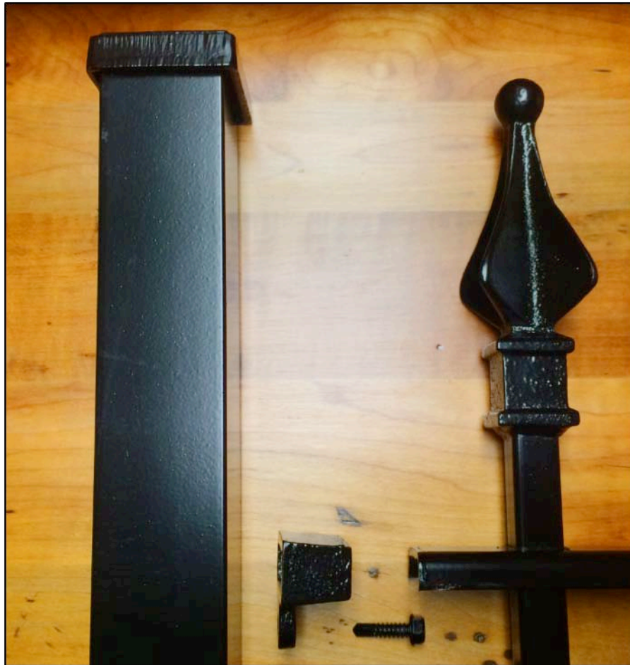
Figure 10 - Main Fence Components: Fence Post, Bracket, Screw, and Fence Panel
